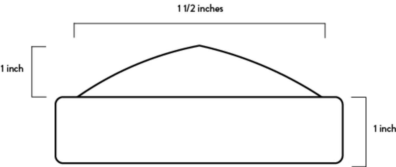
(Side View)
